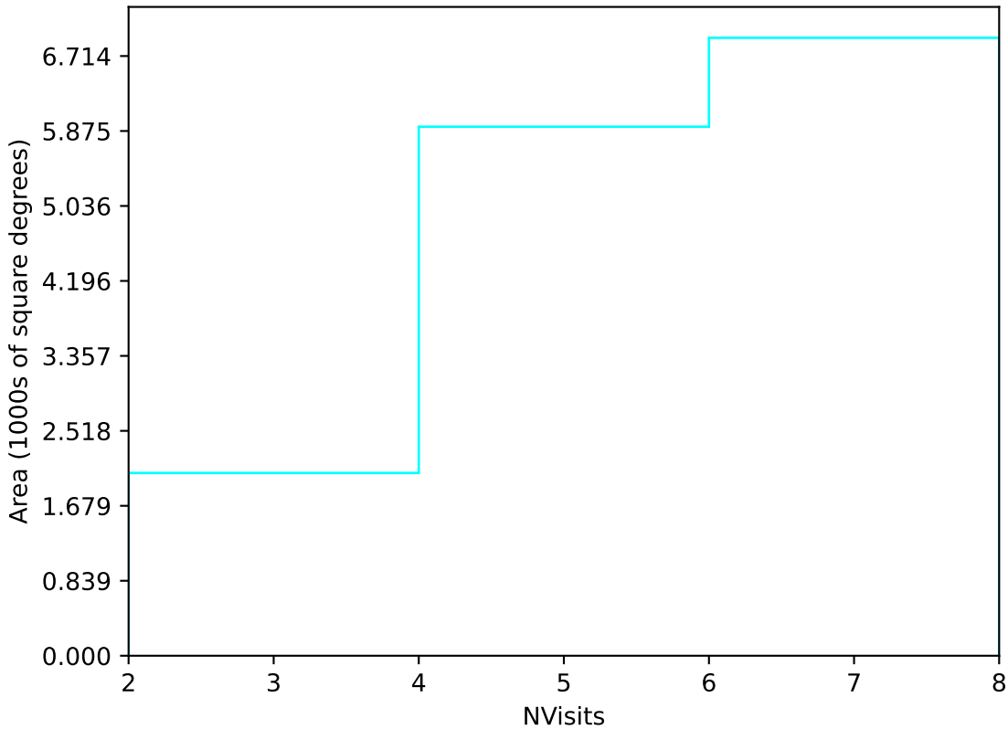
early_u_fpextra2.0_v3.4_10yrs Yr 1 u band: NVisits
