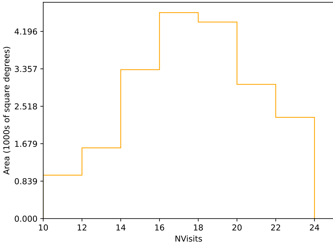
early_u_fpextra2.0_v3.4_10yrs Yr 1 r band: NVisits
