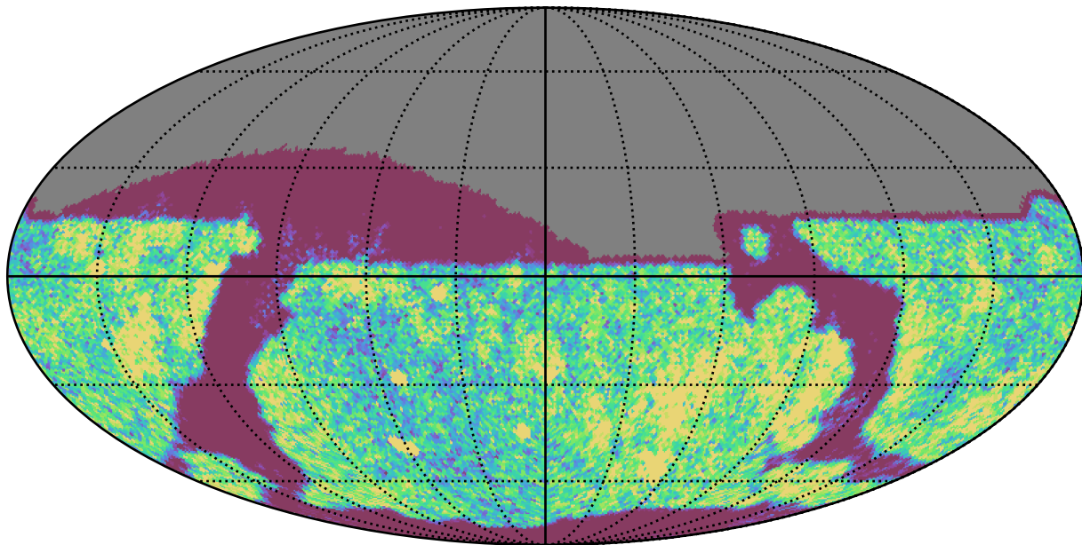
early_u_fpextra2.0_v3.4_10yrs Yr 1 i band: NVisits
