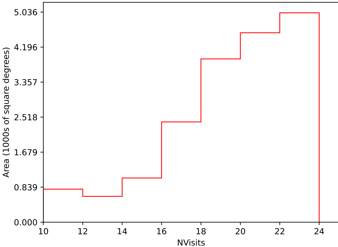
early_u_fpextra2.0_v3.4_10yrs Yr 1 i band: NVisits
