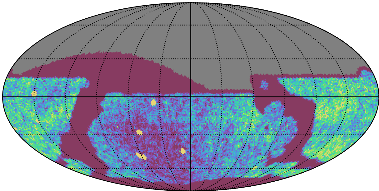
early_u_fpextra2.0_v3.4_10yrs Yr 1 all bands: NVisits
