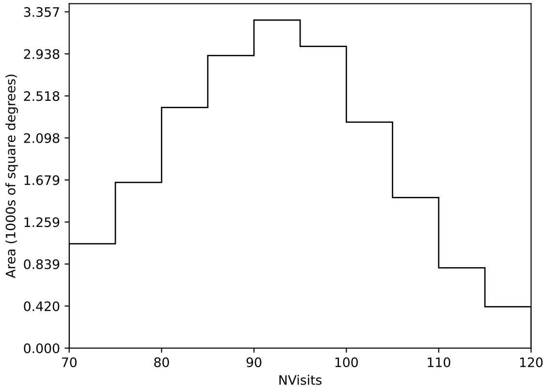
early_u_fpextra2.0_v3.4_10yrs Yr 1 all bands: NVisits
