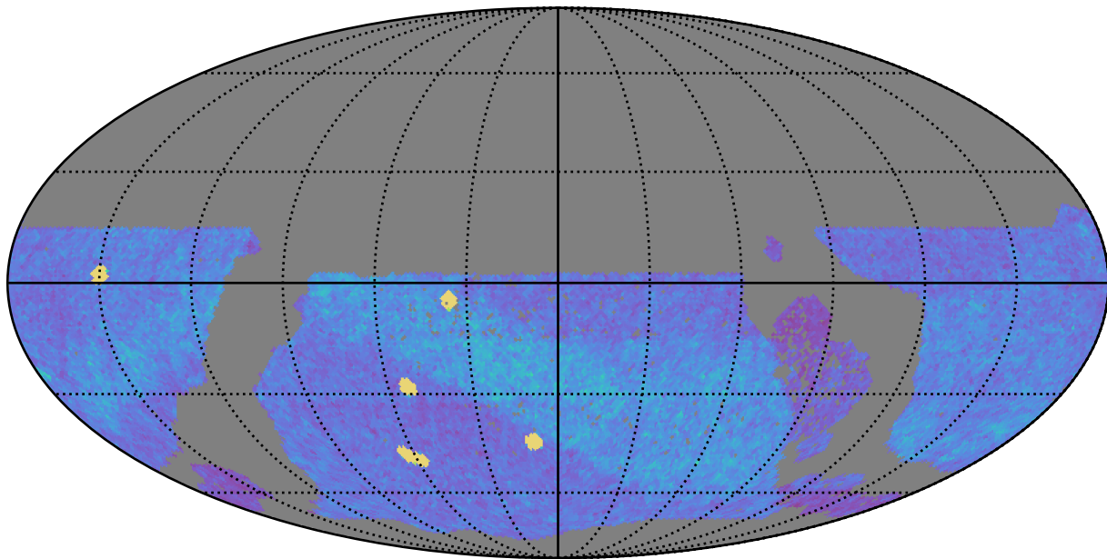
early_u_fpextra2.0_v3.4_10yrs WFD z band: NVisits
