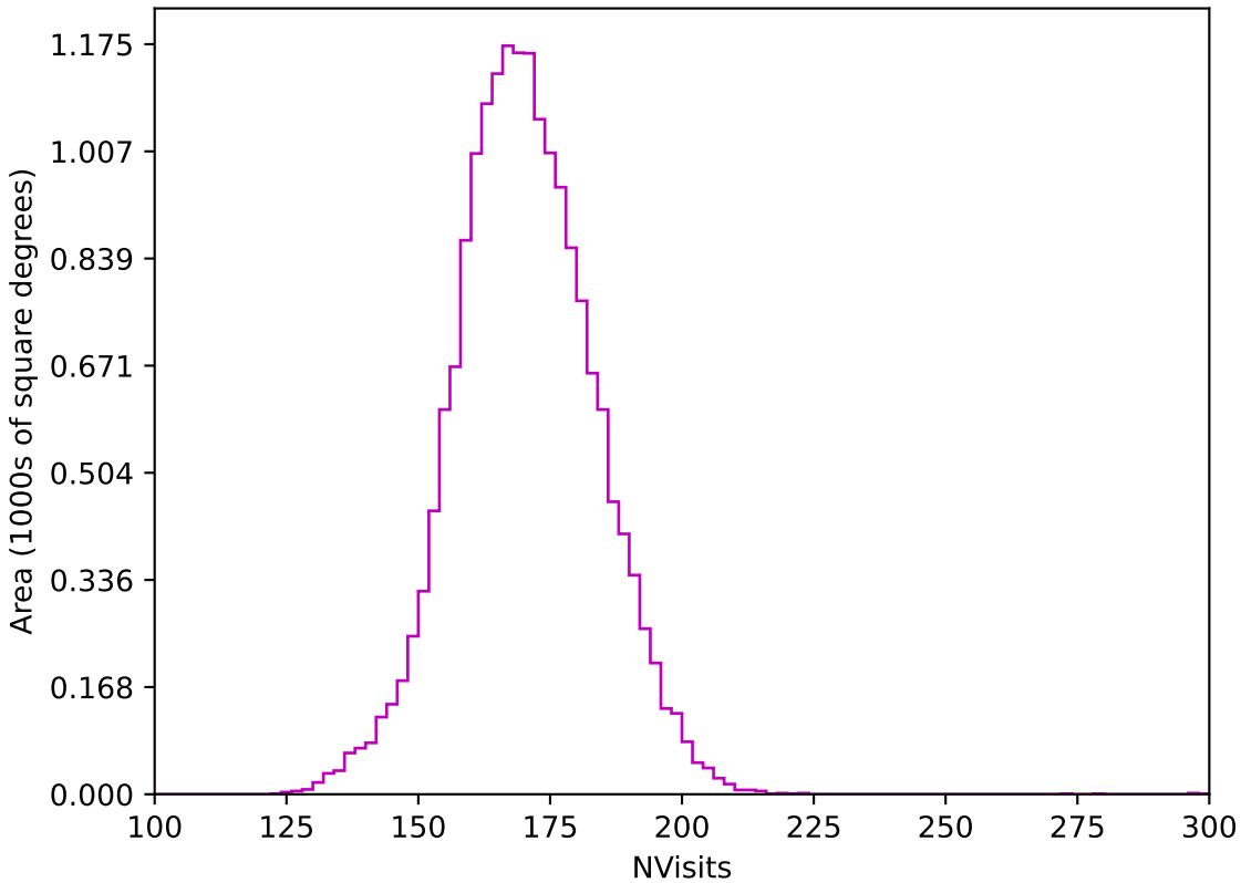
early_u_fpextra2.0_v3.4_10yrs WFD z band: NVisits
