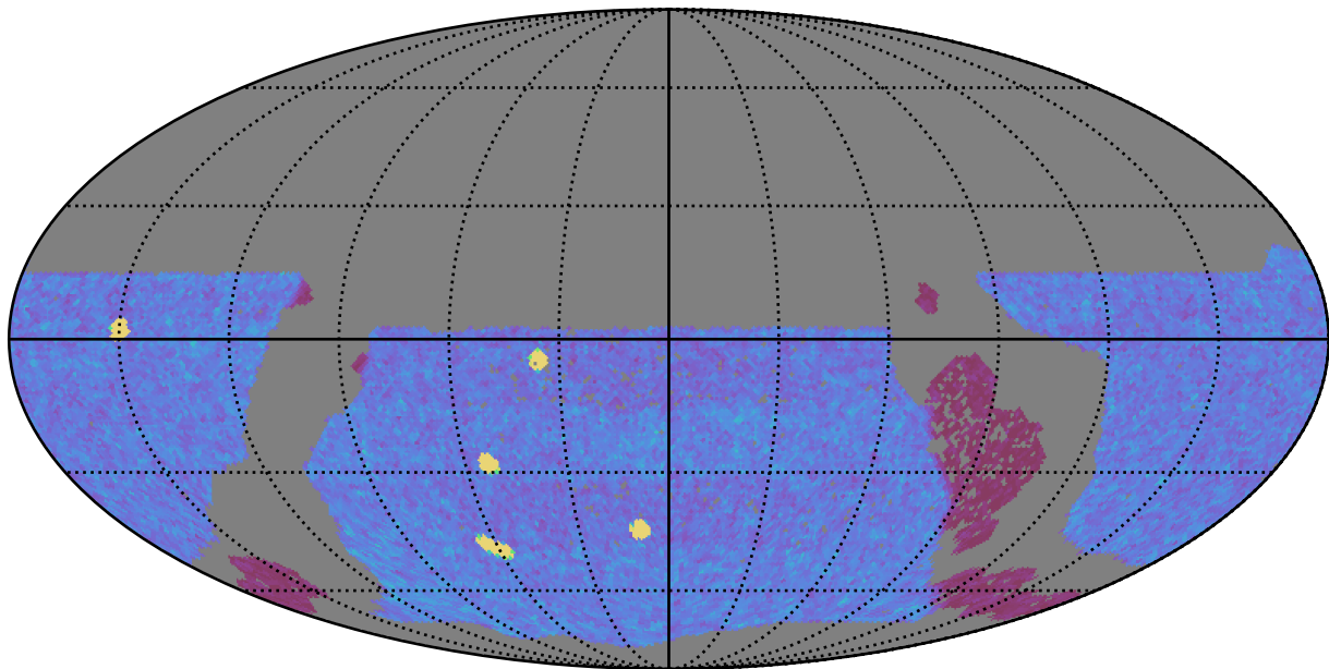
early_u_fpextra2.0_v3.4_10yrs WFD y band: NVisits
