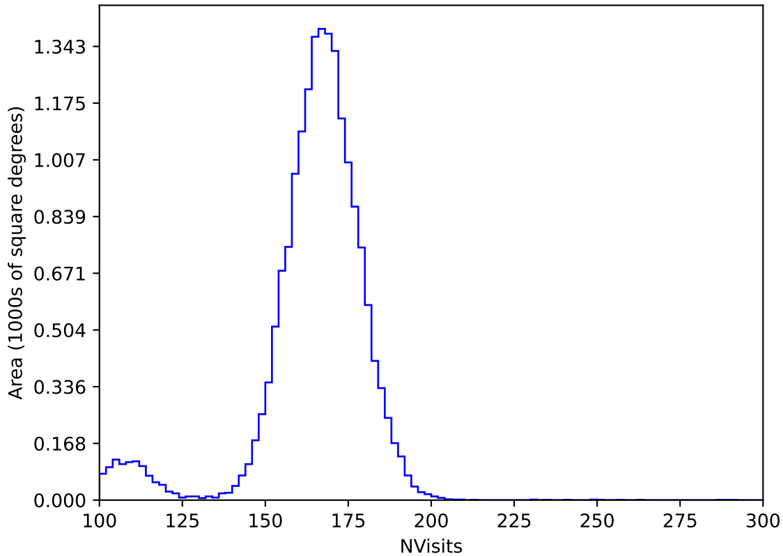
early_u_fpextra2.0_v3.4_10yrs WFD y band: NVisits
