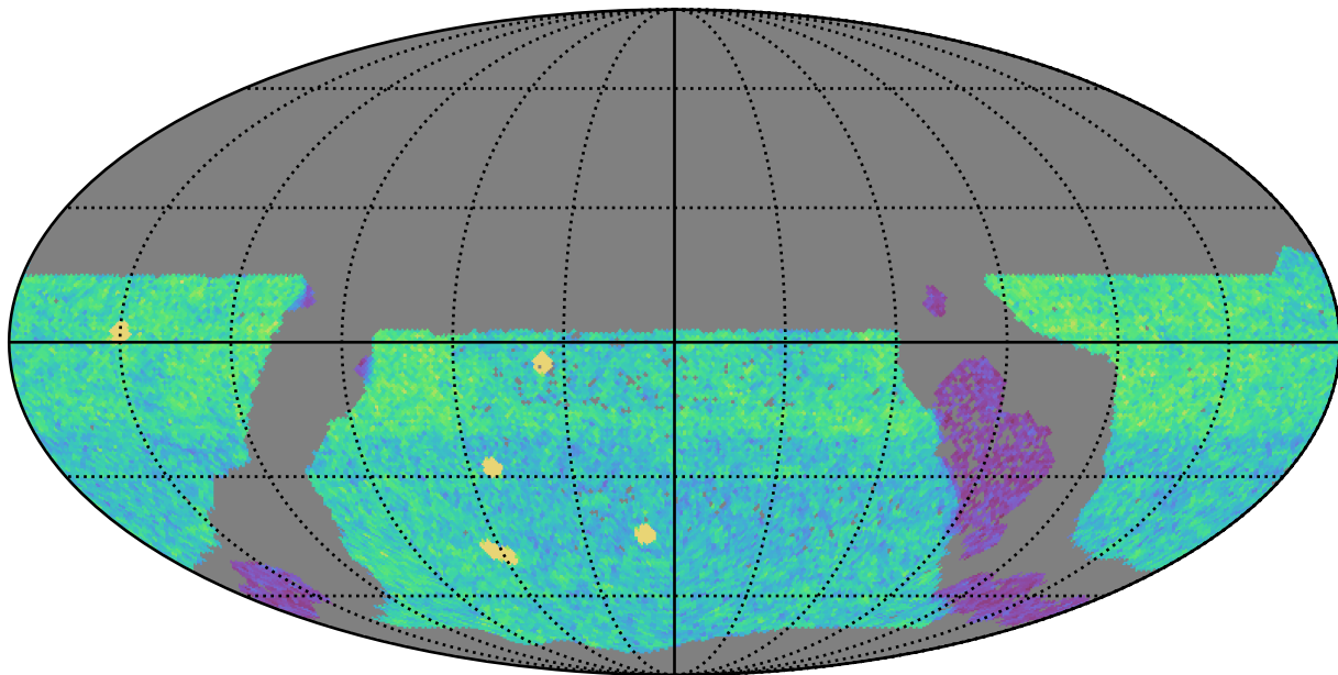
early_u_fpextra2.0_v3.4_10yrs WFD u band: NVisits
