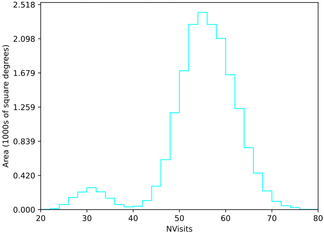
early_u_fpextra2.0_v3.4_10yrs WFD u band: NVisits
