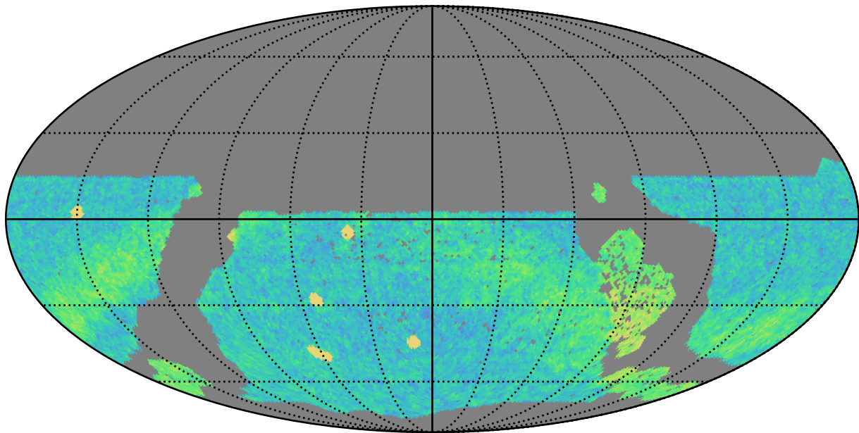
early_u_fpextra2.0_v3.4_10yrs WFD r band: NVisits
