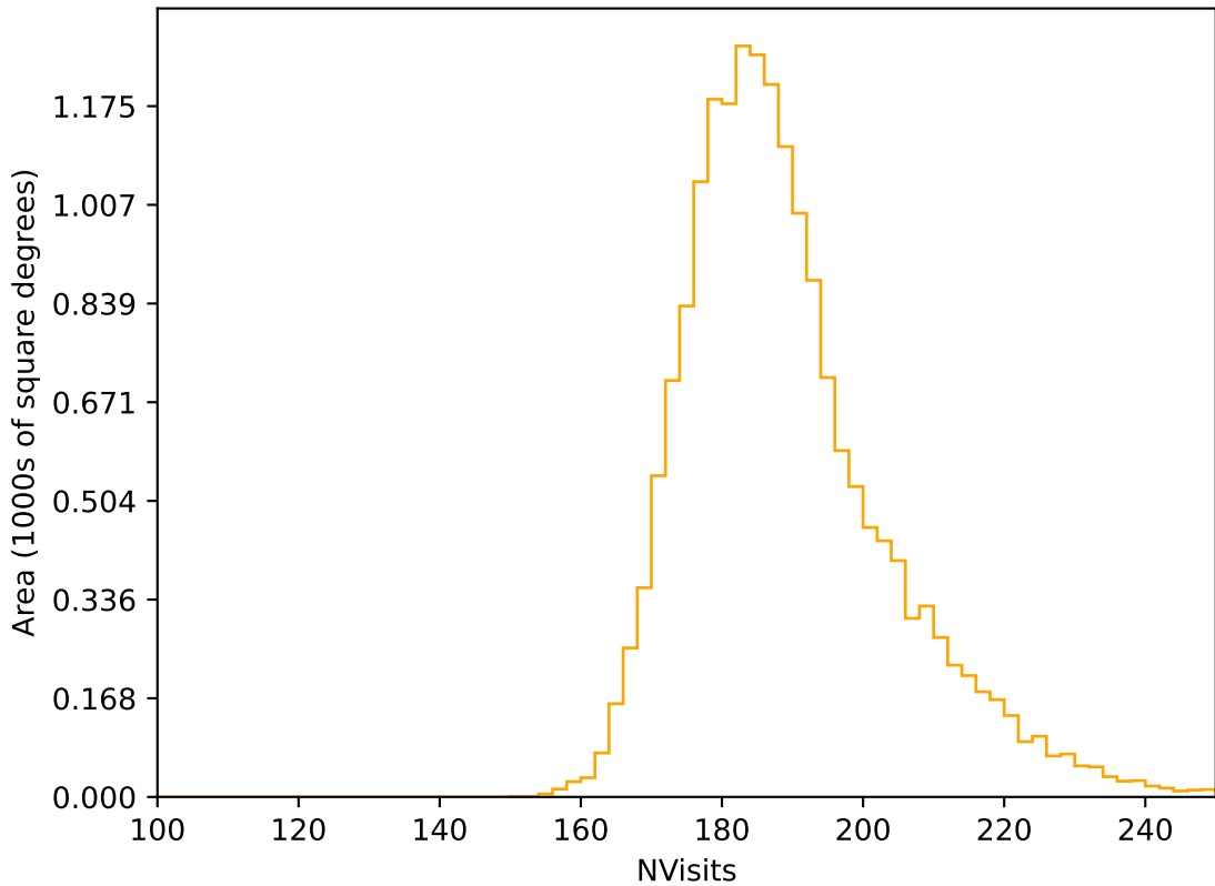
early_u_fpextra2.0_v3.4_10yrs WFD r band: NVisits
