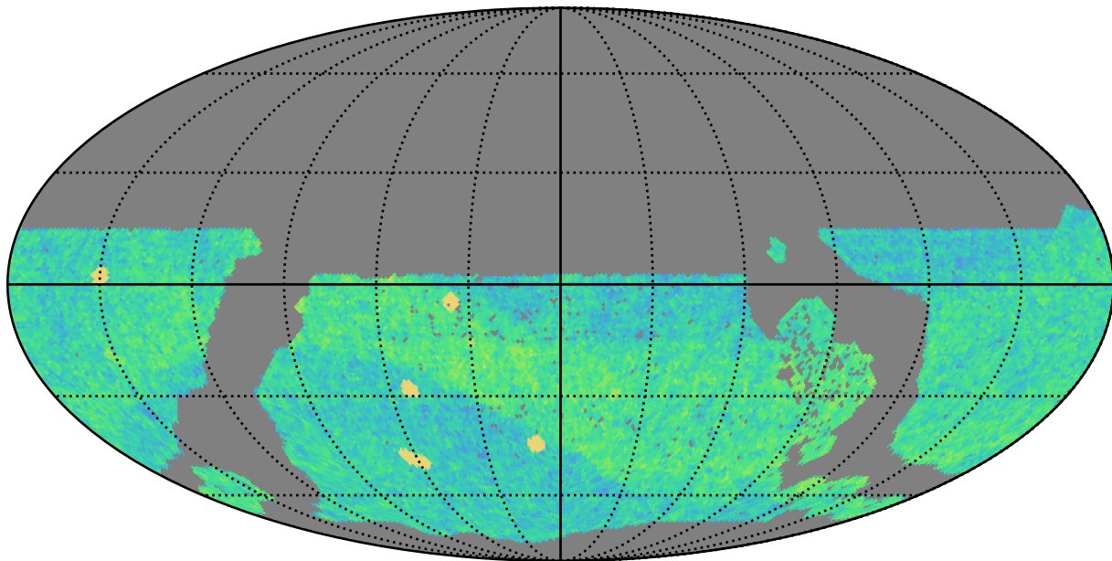
early_u_fpextra2.0_v3.4_10yrs WFD i band: NVisits
