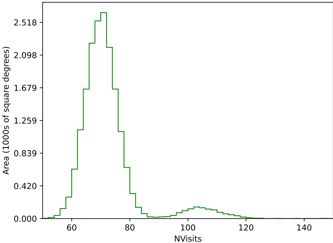
early_u_fpextra2.0_v3.4_10yrs WFD g band: NVisits
