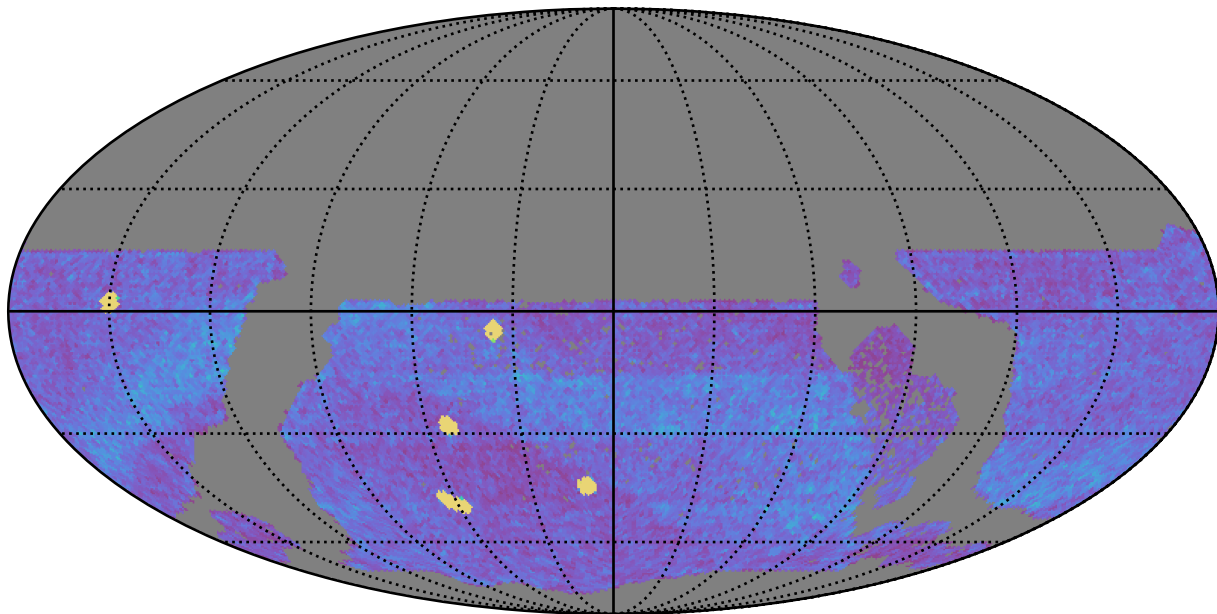
early_u_fpextra2.0_v3.4_10yrs WFD all bands: NVisits
