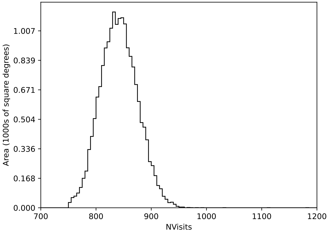
early_u_fpextra2.0_v3.4_10yrs WFD all bands: NVisits
