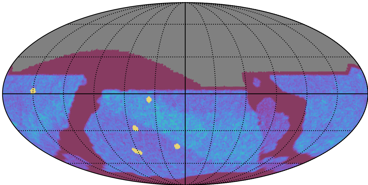
early_u_fpextra2.0_v3.4_10yrs All sky z band: NVisits
