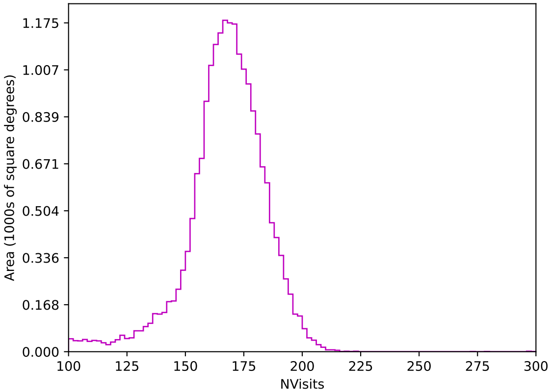
early_u_fpextra2.0_v3.4_10yrs All sky z band: NVisits
