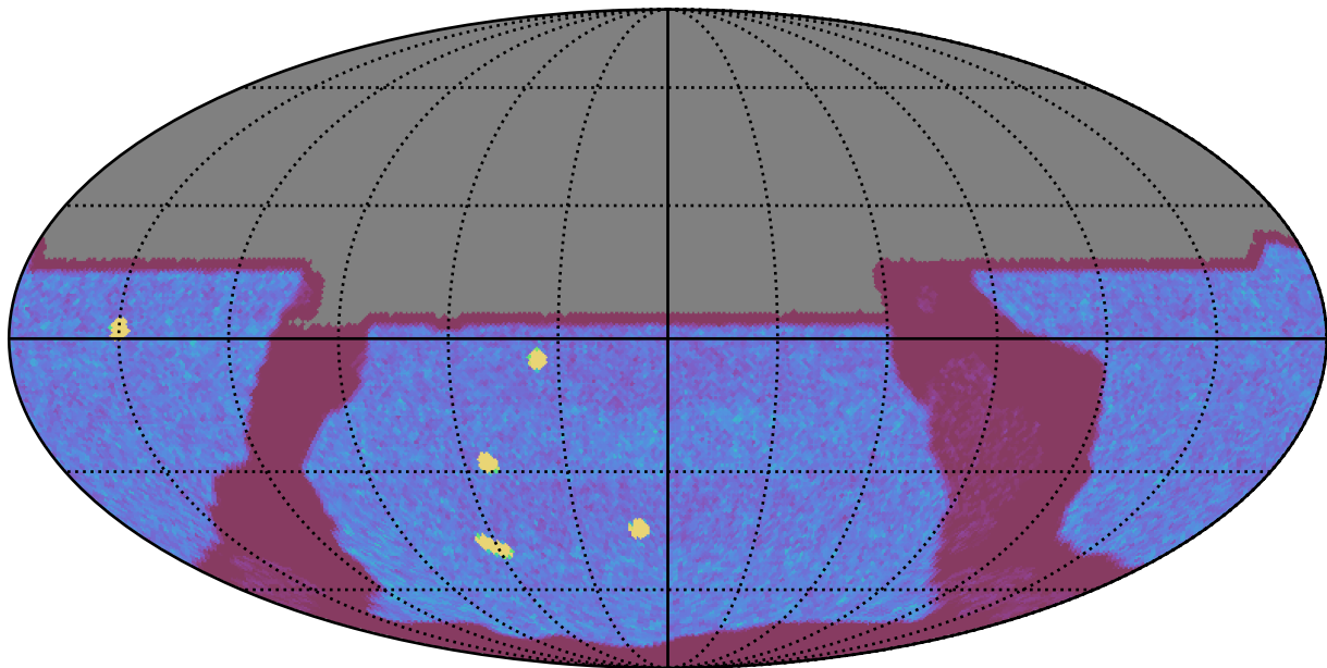
early_u_fpextra2.0_v3.4_10yrs All sky y band: NVisits
