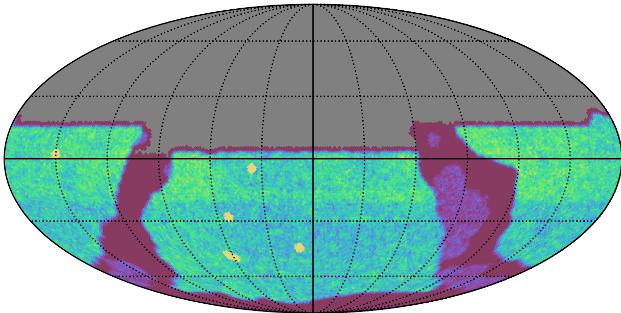
early_u_fpextra2.0_v3.4_10yrs All sky u band: NVisits
