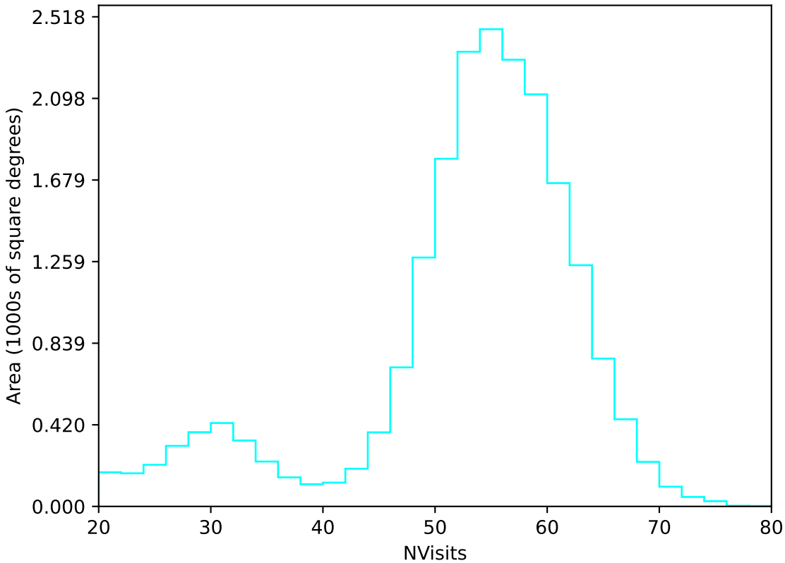
early_u_fpextra2.0_v3.4_10yrs All sky u band: NVisits
