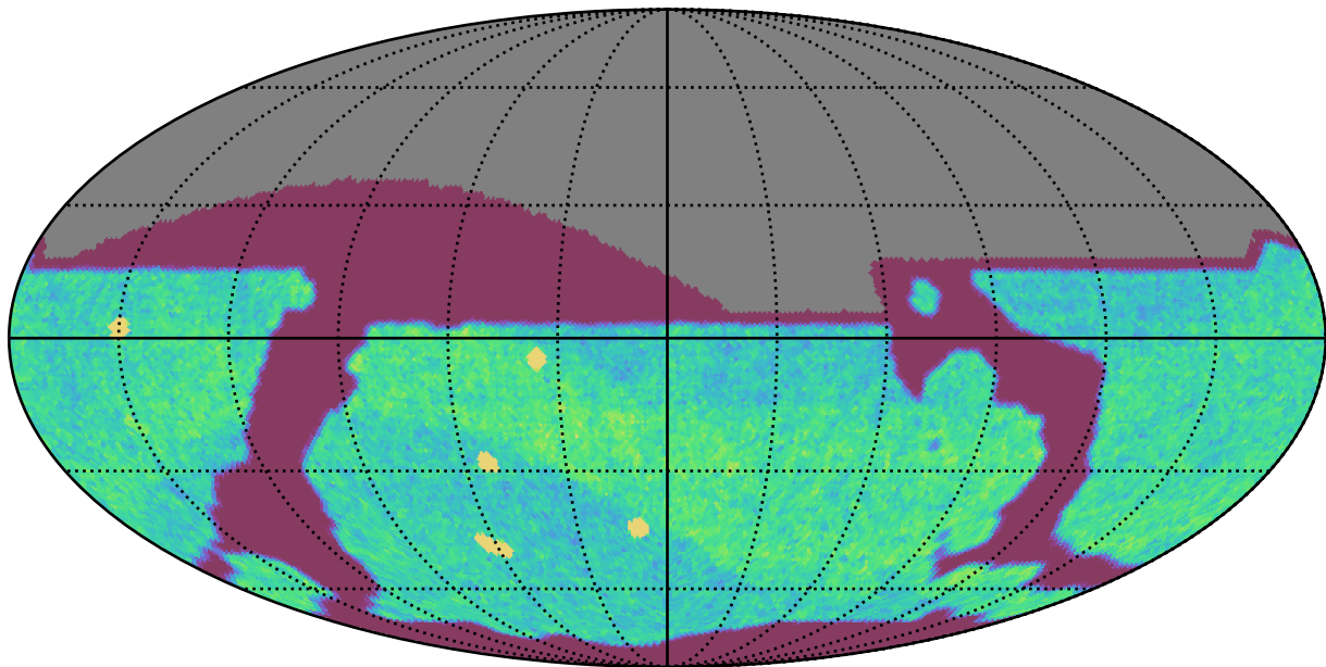
early_u_fpextra2.0_v3.4_10yrs All sky i band: NVisits
