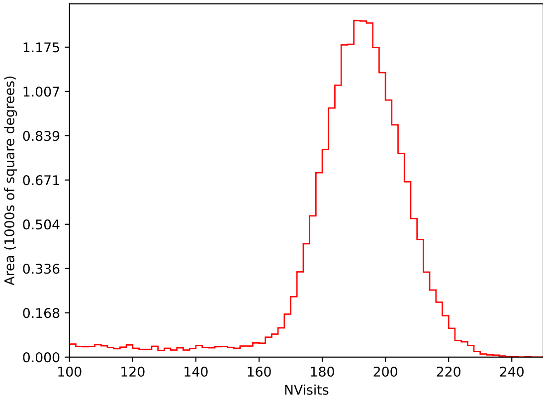
early_u_fpextra2.0_v3.4_10yrs All sky i band: NVisits
