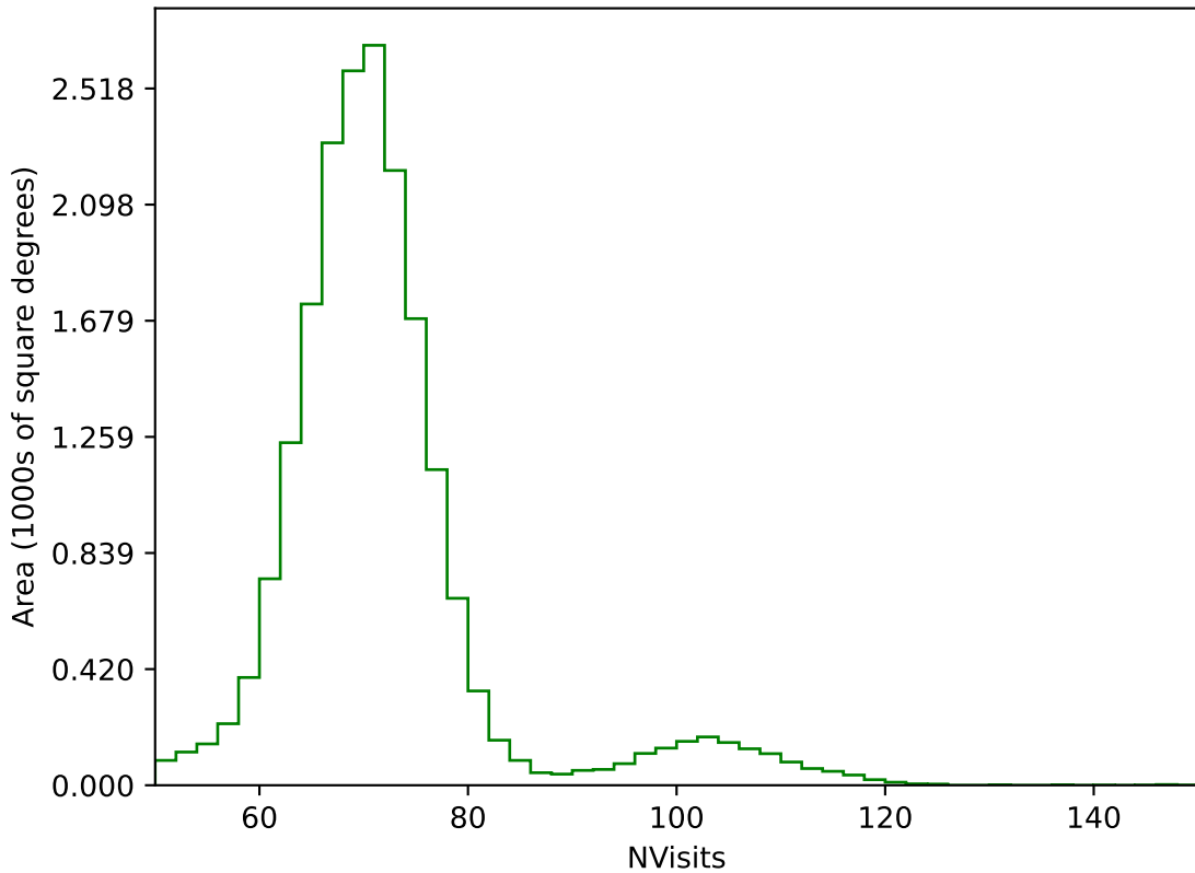
early_u_fpextra2.0_v3.4_10yrs All sky g band: NVisits
