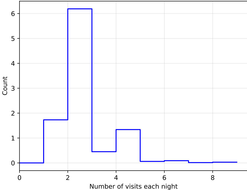
early_u_fpextra2.0_v3.4_10yrs All sky: NVisitsPerNight
