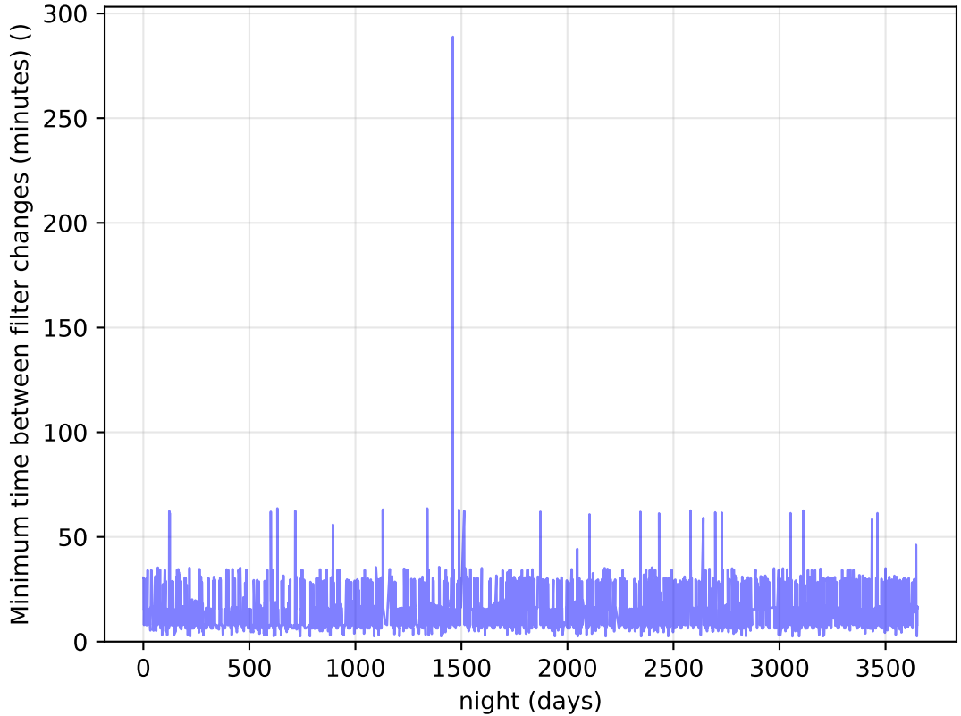
early_u_fpxtra2.0_v3.4_10yrs Per Night: Minimum time between filter changes (minutes)
