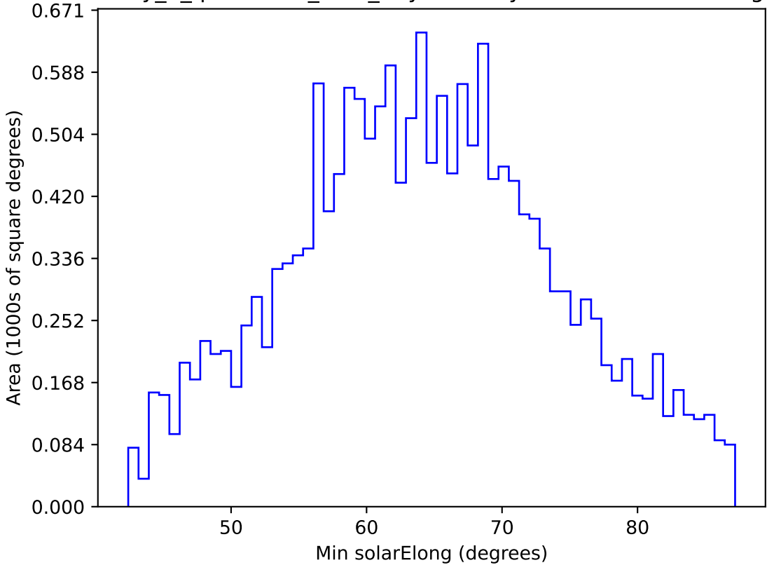
early_u_fpextra2.0_v3.4_10yrs WFD y band: Min solarElong
