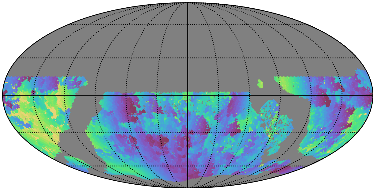
early_u_fpextra2.0_v3.4_10yrs WFD u band: Min solarElong
