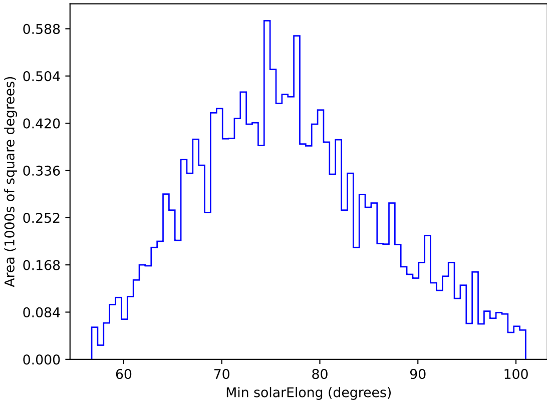
early_u_fpextra2.0_v3.4_10yrs WFD u band: Min solarElong
