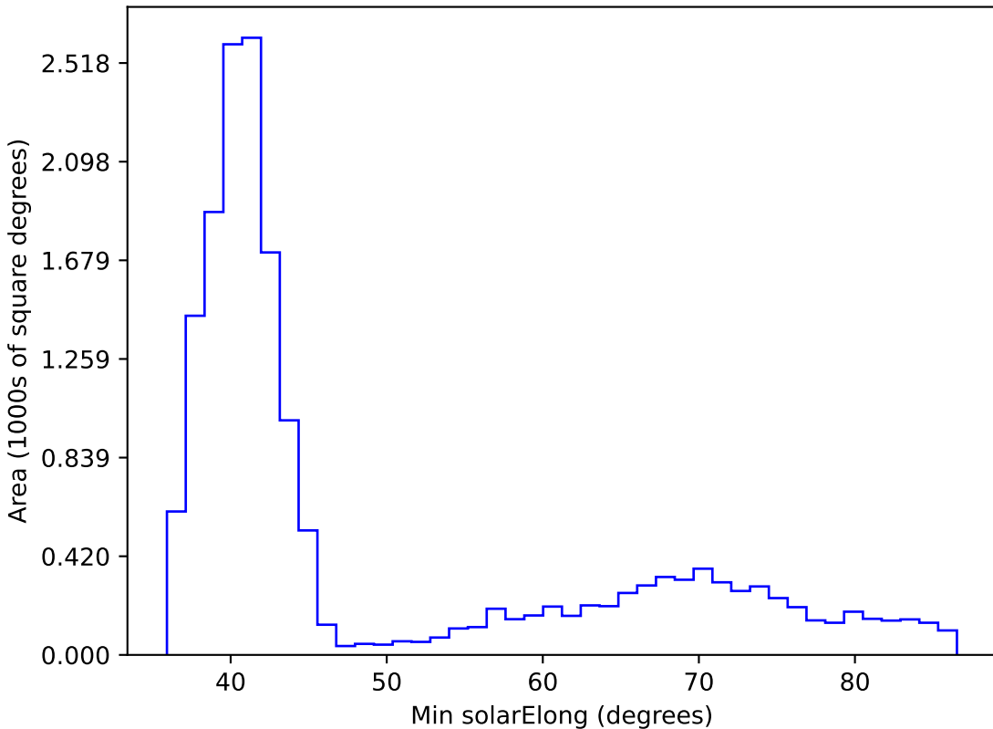
early_u_fpextra2.0_v3.4_10yrs WFD i band: Min solarElong
