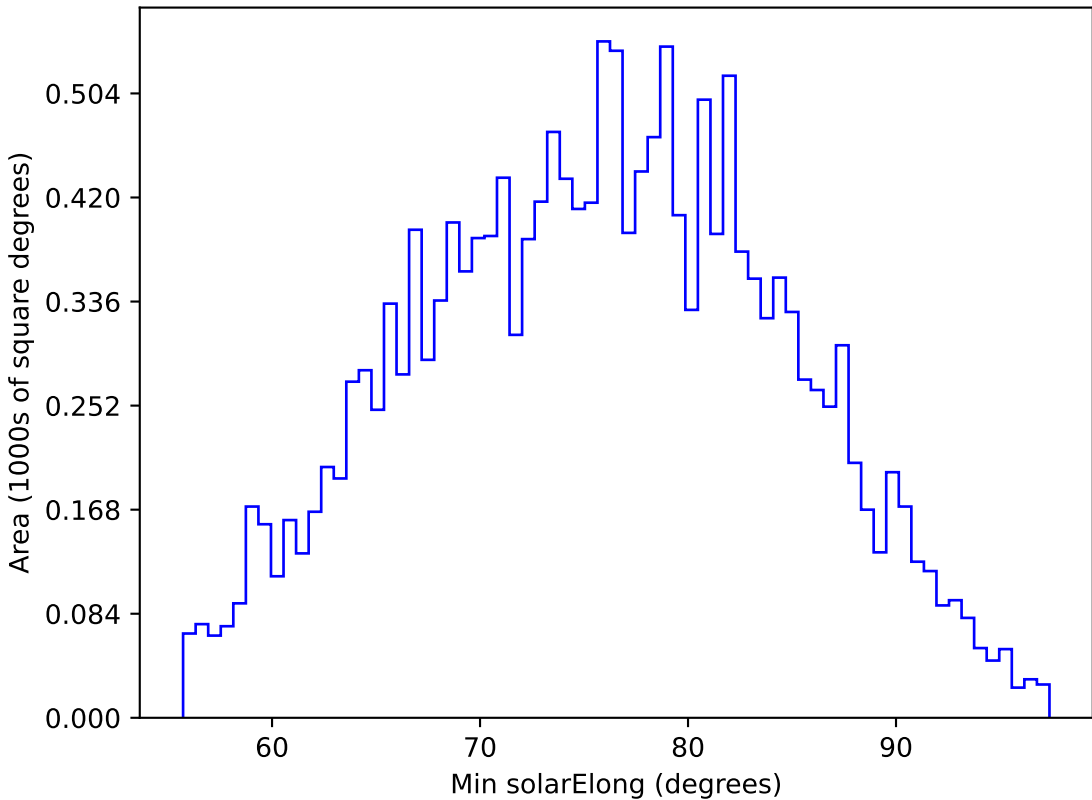
early_u_fpextra2.0_v3.4_10yrs WFD g band: Min solarElong
