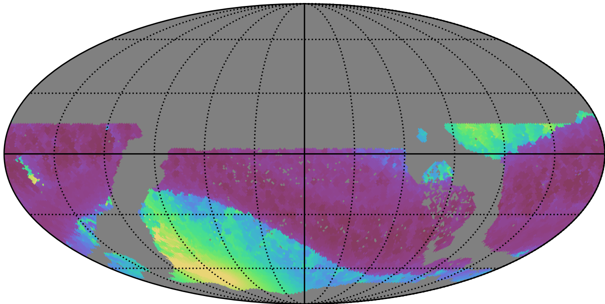
early_u_fpextra2.0_v3.4_10yrs WFD all bands: Min solarElong
