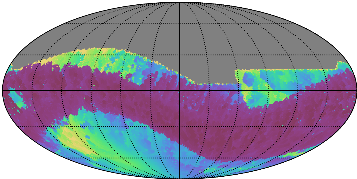
early_u_fpextra2.0_v3.4_10yrs All sky z band: Min solarElong
