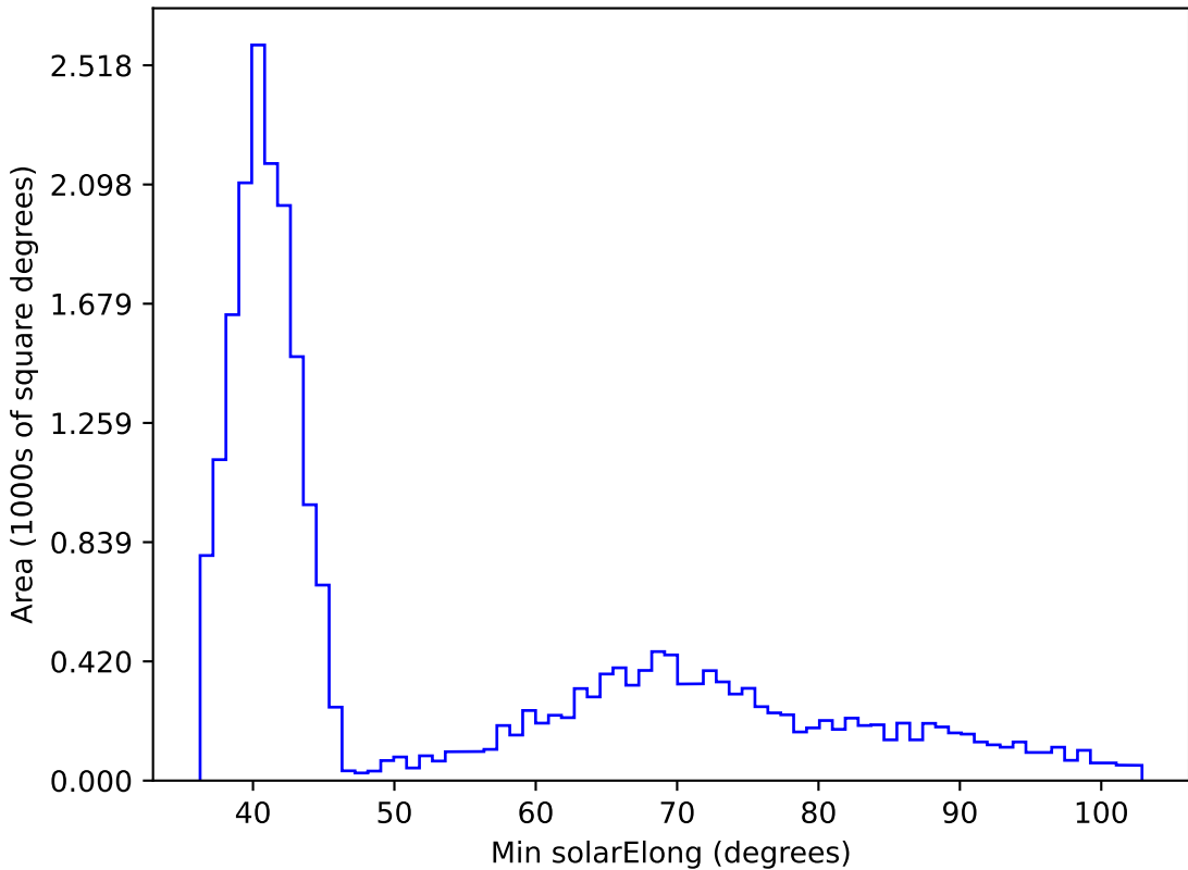
early_u_fpextra2.0_v3.4_10yrs All sky z band: Min solarElong
