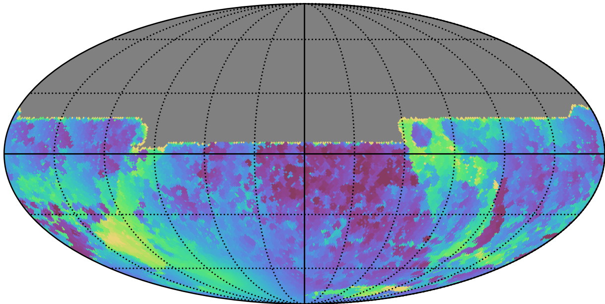
early_u_fpextra2.0_v3.4_10yrs All sky y band: Min solarElong
