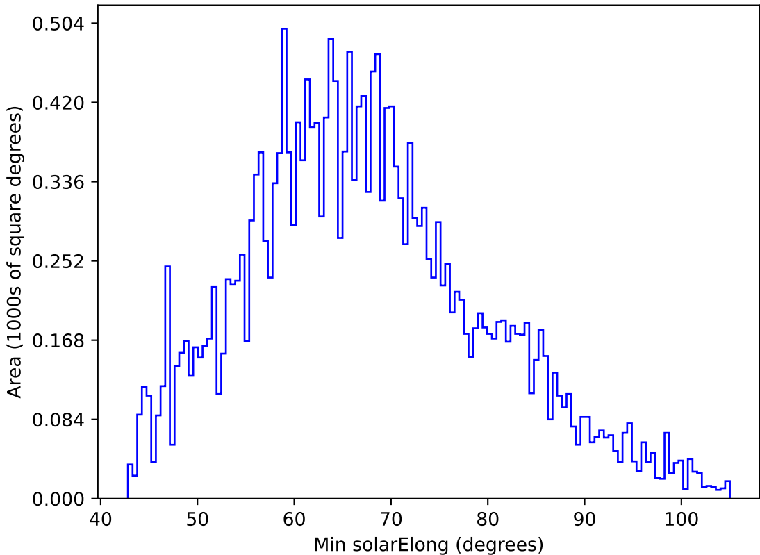
early_u_fpextra2.0_v3.4_10yrs All sky y band: Min solarElong
