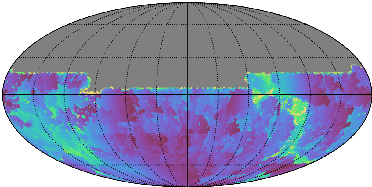
early_u_fpextra2.0_v3.4_10yrs All sky u band: Min solarElong
