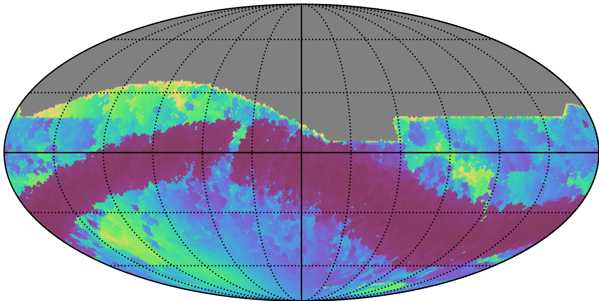
early_u_fpextra2.0_v3.4_10yrs All sky r band: Min solarElong
