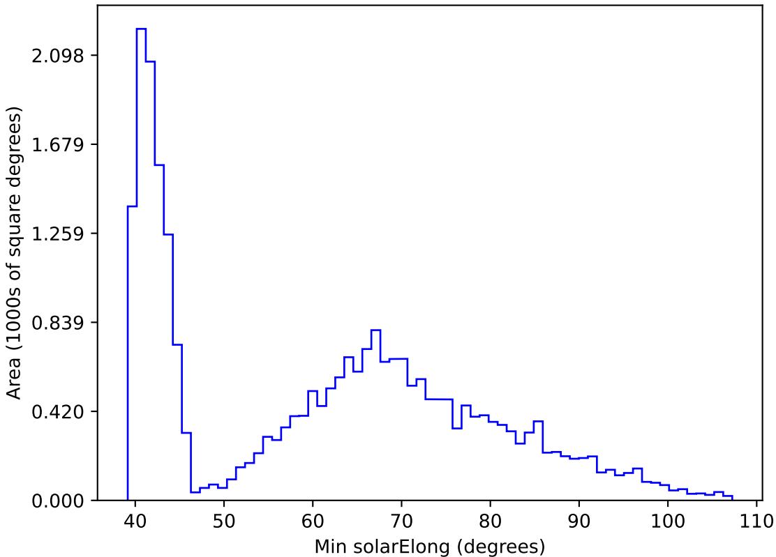
early_u_fpextra2.0_v3.4_10yrs All sky r band: Min solarElong
