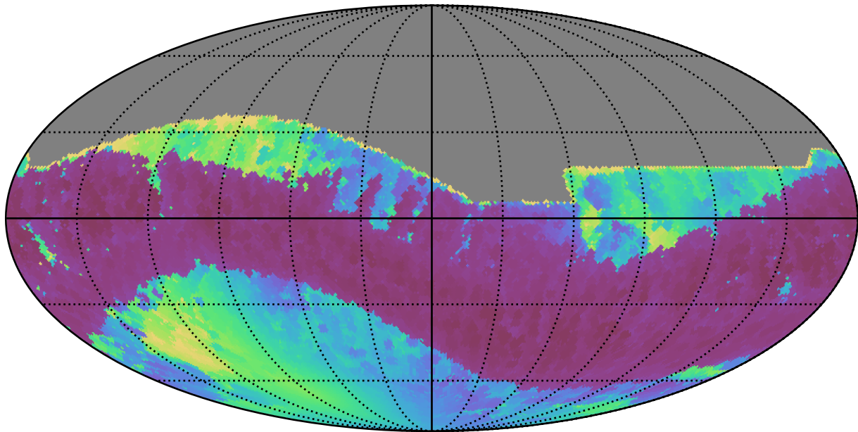
early_u_fpextra2.0_v3.4_10yrs All sky i band: Min solarElong
