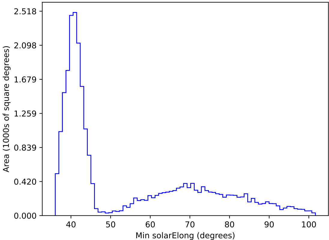
early_u_fpextra2.0_v3.4_10yrs All sky i band: Min solarElong
