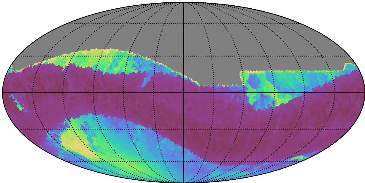
early_u_fpextra2.0_v3.4_10yrs All sky all bands: Min solarElong
