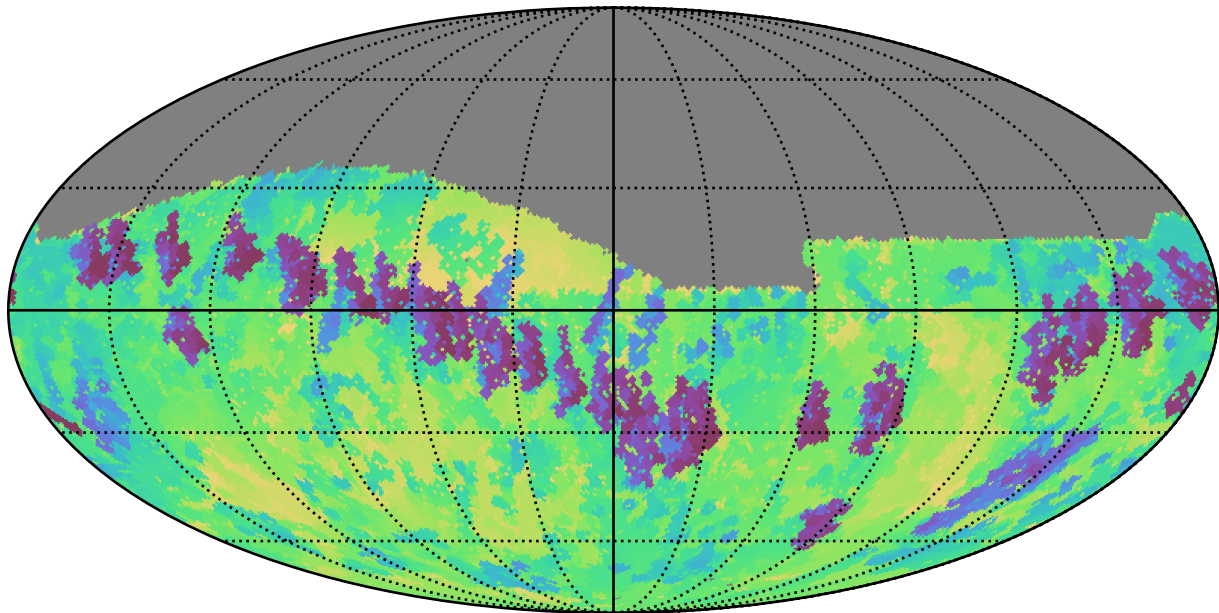
early_u_fpextra2.0_v3.4_10yrs Yr 1 z band: Min skyBrightness
