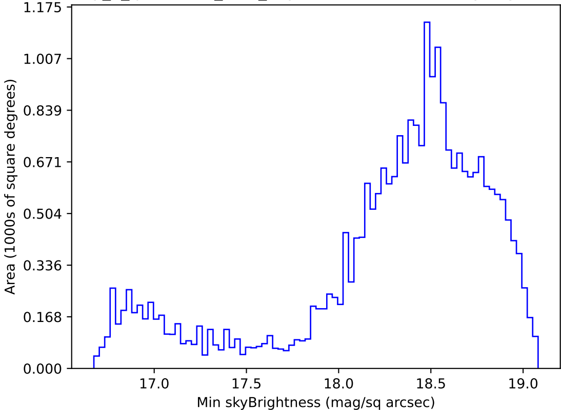
early_u_fpextra2.0_v3.4_10yrs Yr 1 z band: Min skyBrightness
