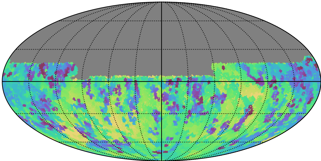
early_u_fpextra2.0_v3.4_10yrs Yr 1 y band: Min skyBrightness
