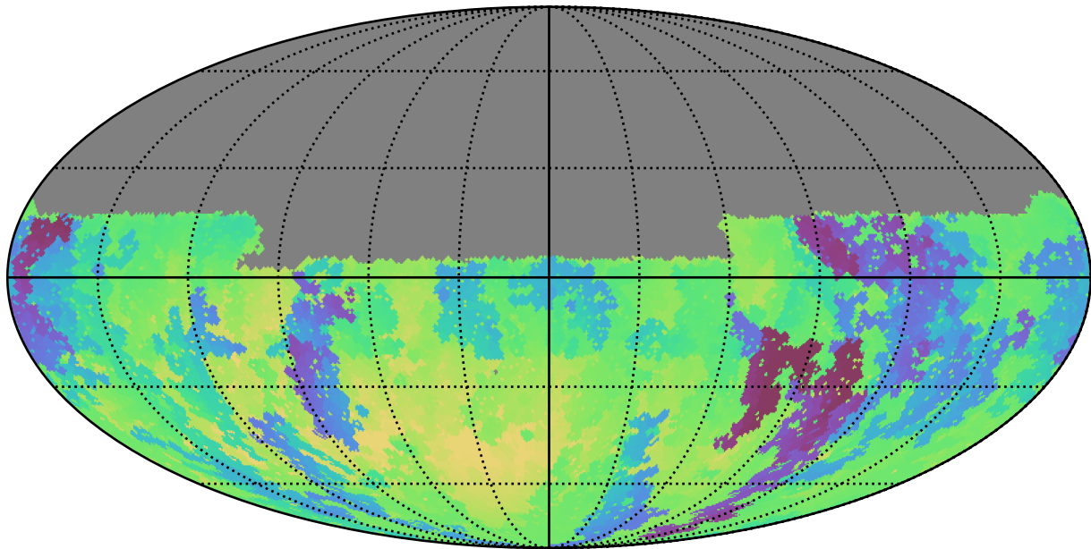
early_u_fpextra2.0_v3.4_10yrs Yr 1 u band: Min skyBrightness
