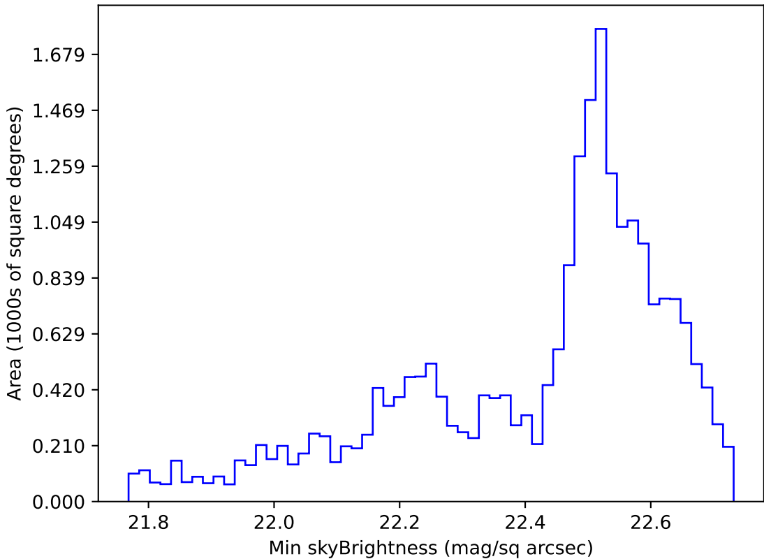
early_u_fpextra2.0_v3.4_10yrs Yr 1 u band: Min skyBrightness
