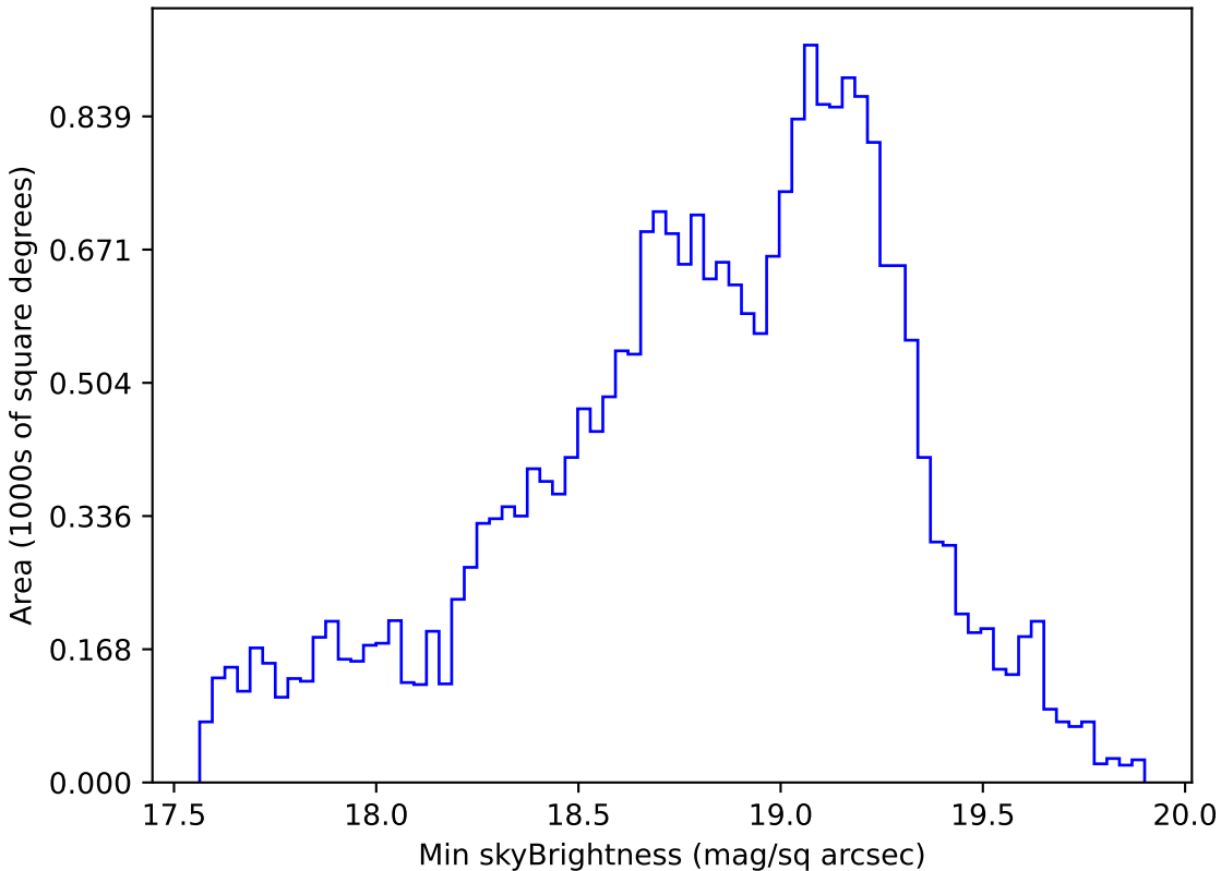
early_u_fpextra2.0_v3.4_10yrs Yr 1 i band: Min skyBrightness
